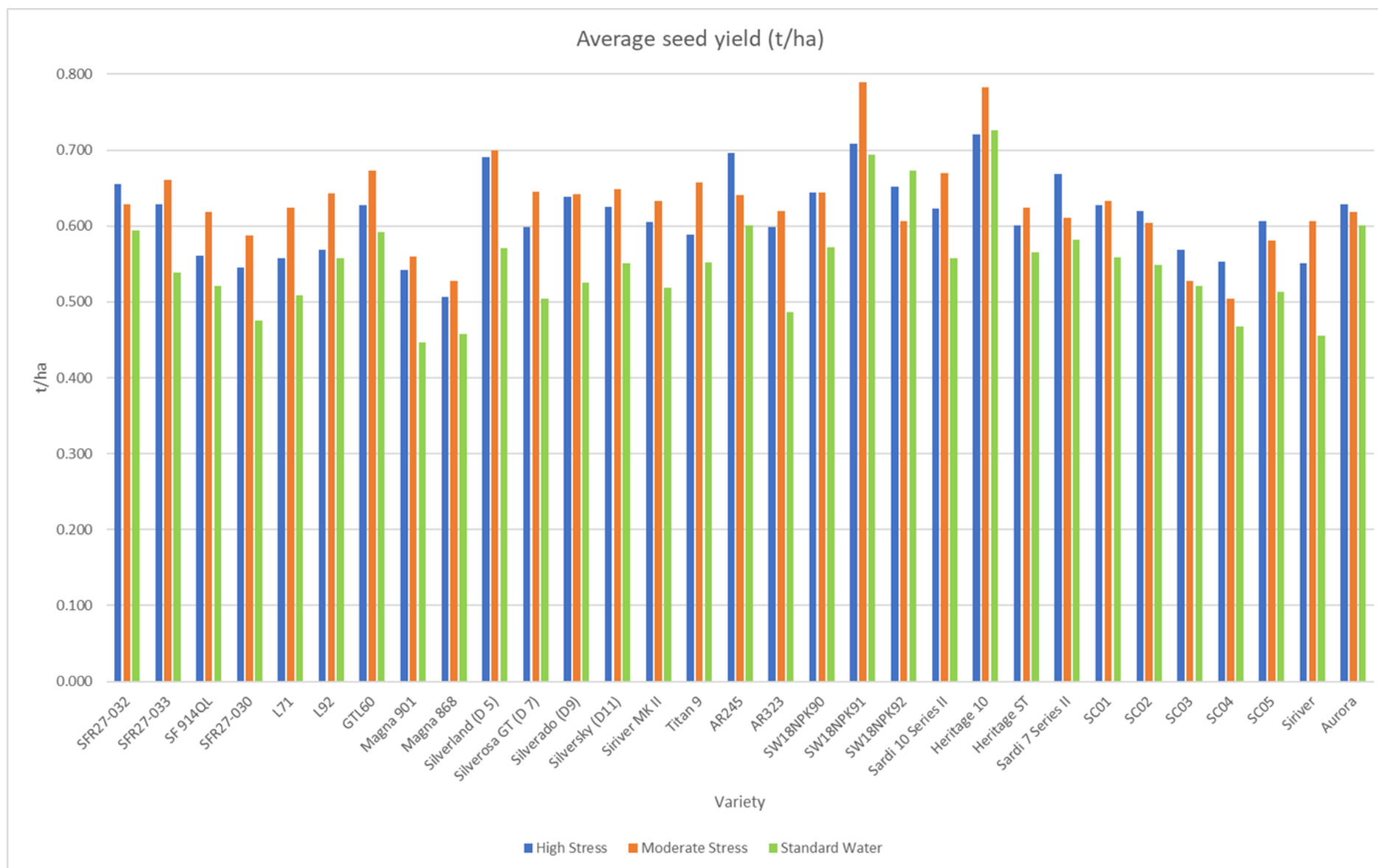
Graph 1 -Average seed yield (t/ha) per variety for each watering strategy
